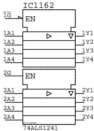
74ALS1241 IC????
