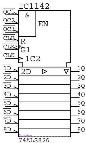
74ALS826 IC????
