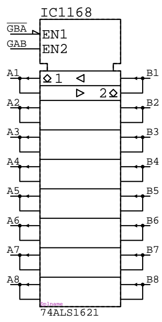
74ALS1621 IC????
