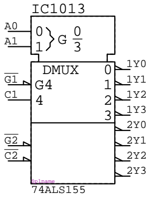
74ALS155 IC????
