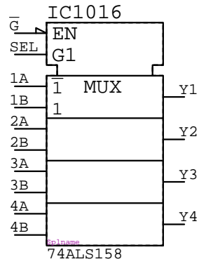
74ALS158 IC????
