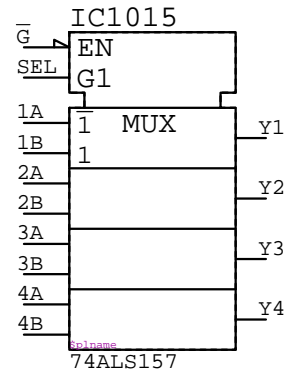
74ALS157 IC????
