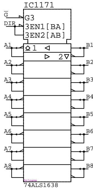
74ALS1638 IC????
