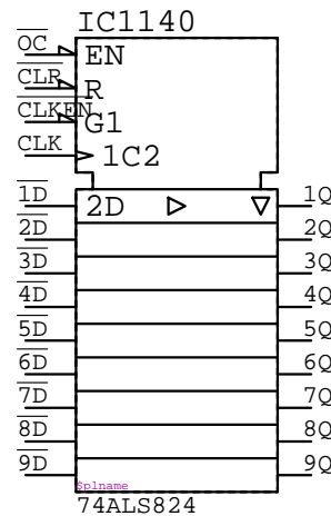
74ALS824 IC????
