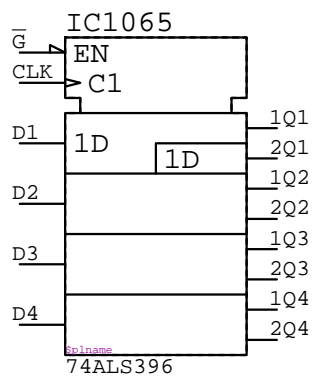
74ALS396 IC????
