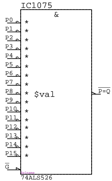
74ALS526 IC?????
