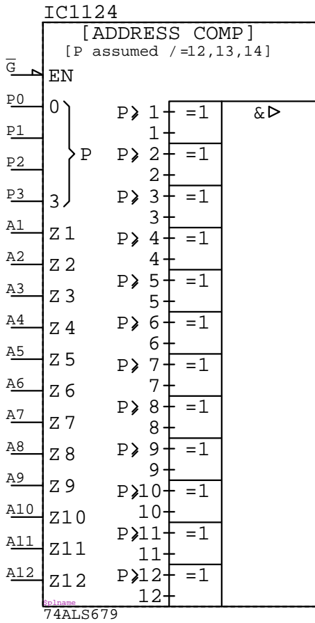
74ALS679 IC????
