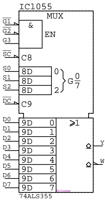
74ALS355 IC????
