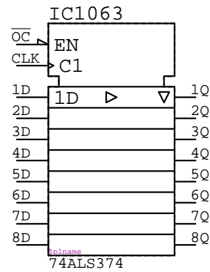
74ALS374 IC????
