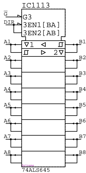
74ALS645 IC?????
