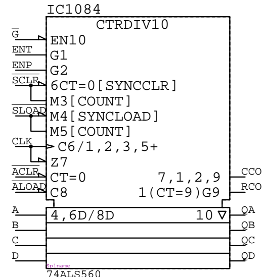
74ALS560 IC?????
