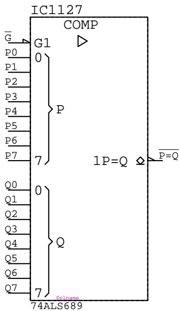
74ALS689 IC????
