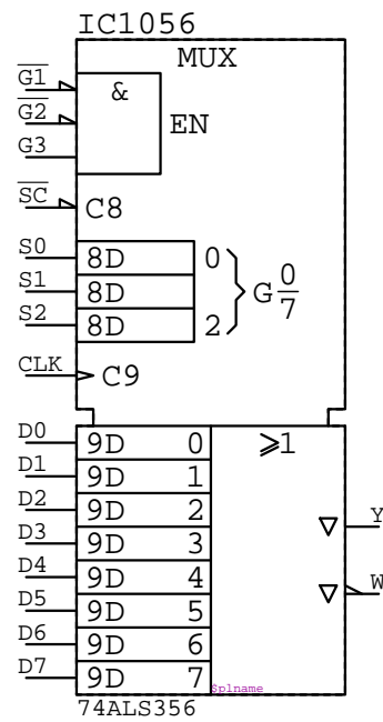
74ALS356 IC????
