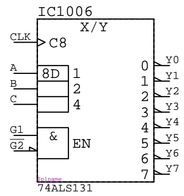
74ALS131 IC????
