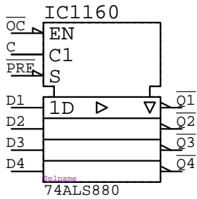
74ALS880 IC????
