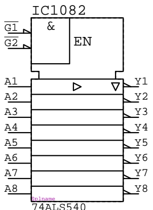
74ALS540 IC?????
