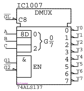
74ALS137 IC????
