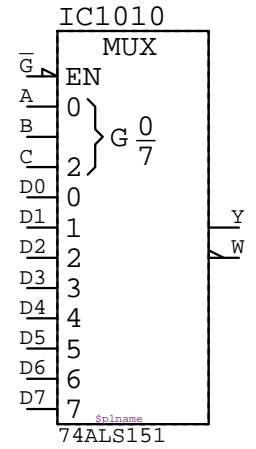
74ALS151 IC????
