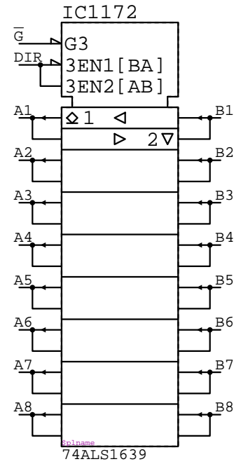
74ALS1639 IC????
