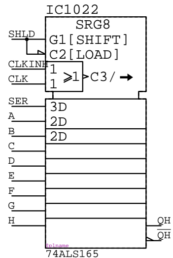
74ALS165 IC????
