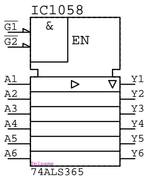
74ALS365 IC????
