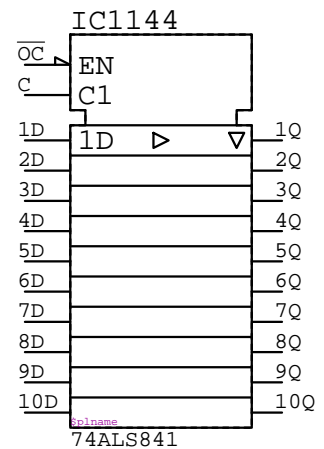
74ALS841 IC????
