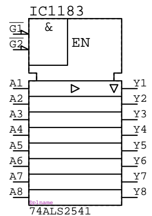
74ALS2541 IC?????
