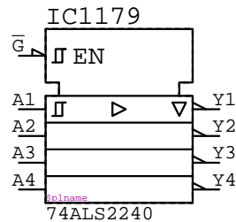
74ALS2240 IC?????
