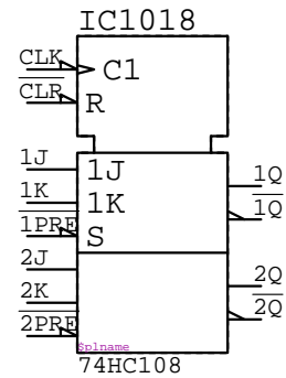
74HC108 IC????
