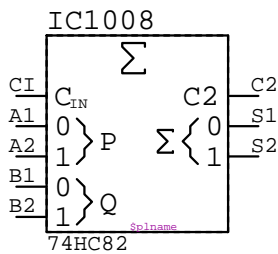
74HC82 IC????
