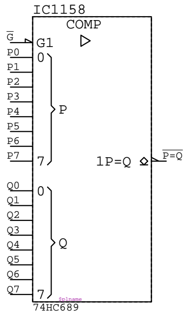
74HC689 IC????
