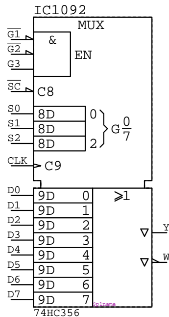
74HC356 IC????
