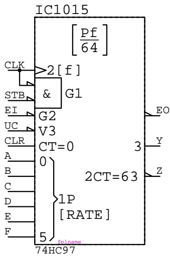
74HC97 IC????
