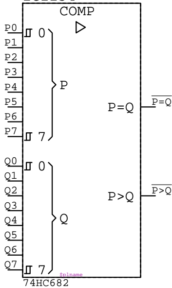
74HC682 IC?????
