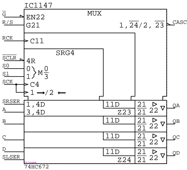
74HC672 IC????
