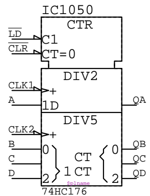
74HC176 IC????
