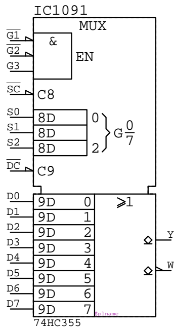
74HC355 IC????
