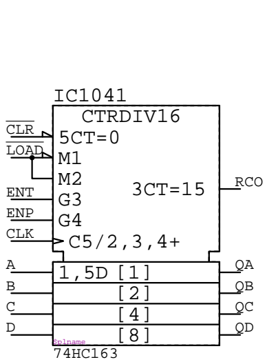
74HC163 IC????
