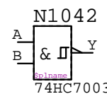
74HC7003 N????
