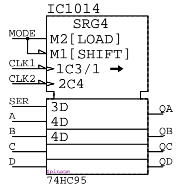
74HC95 IC????
