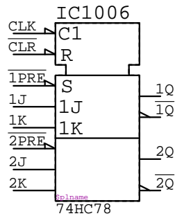
74HC78 IC????
