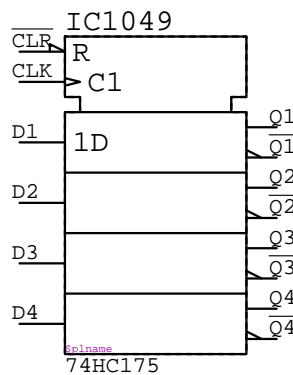
74HC175 IC????
