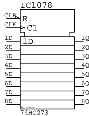
74HC273 IC?????
