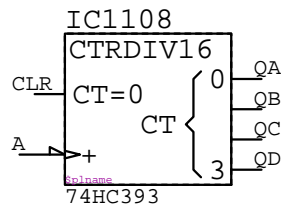
74HC393 IC????
