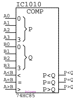
74HC85 IC????
