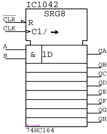
74HC164 IC????
