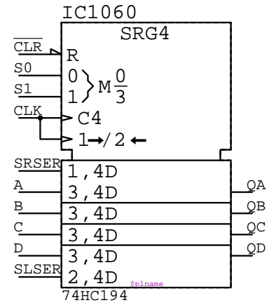
74HC194 IC?????
