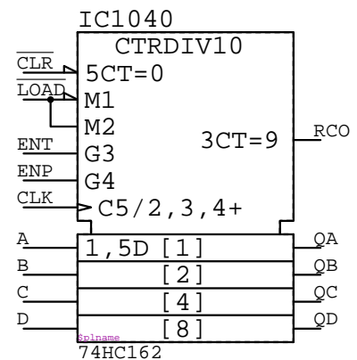
74HC162
