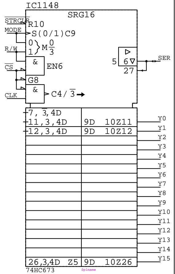
74HC673 IC????
