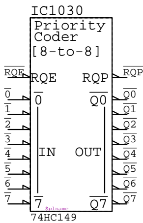
74HC149
