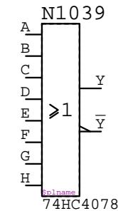
74HC4078 N????
