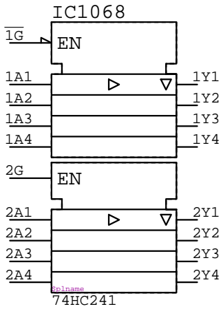
74HC241 IC????
