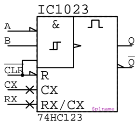
74HC123 IC????
