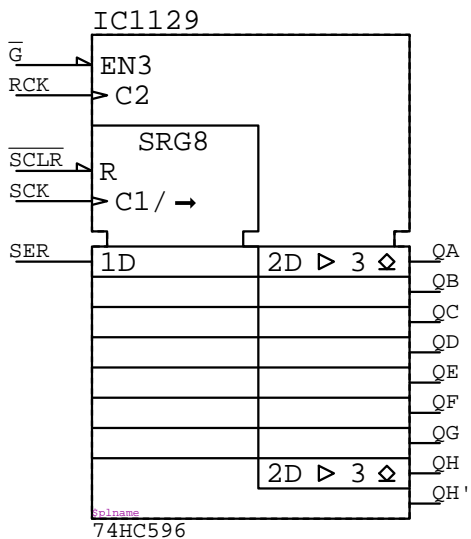
74HC596 IC????
