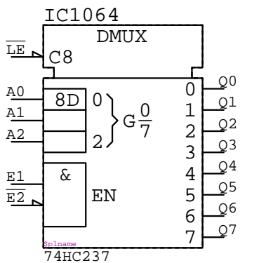
74HC237 IC?????
