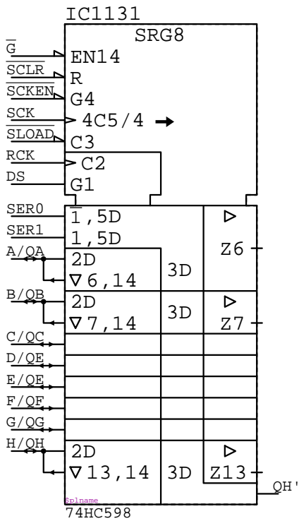
74HC598 IC?????
