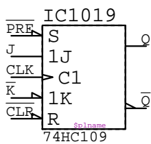
74HC109 IC????
