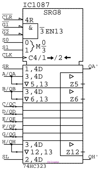
74HC323 IC????
