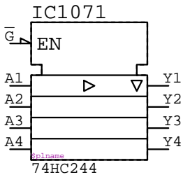
74HC244 IC????
