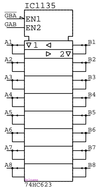
74HC623 IC?????
