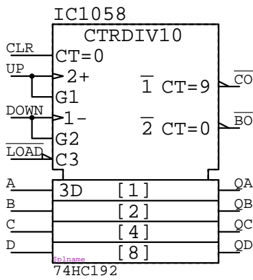
74HC192 IC?????
