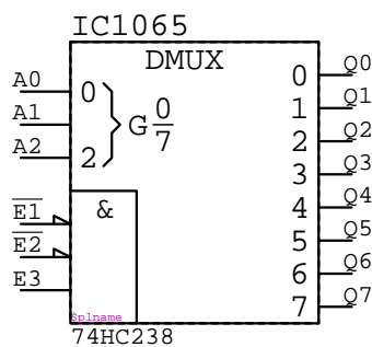
74HC238 IC?????
