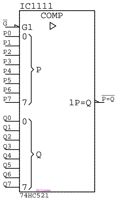
74HC521 IC?????
