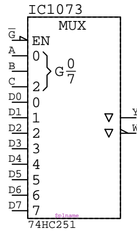
74HC251 IC????
