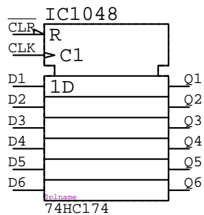
74HC174 IC????
