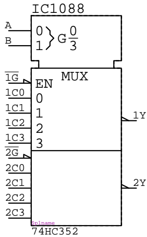
74HC352 IC????
