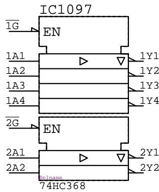
74HC368 IC?????
