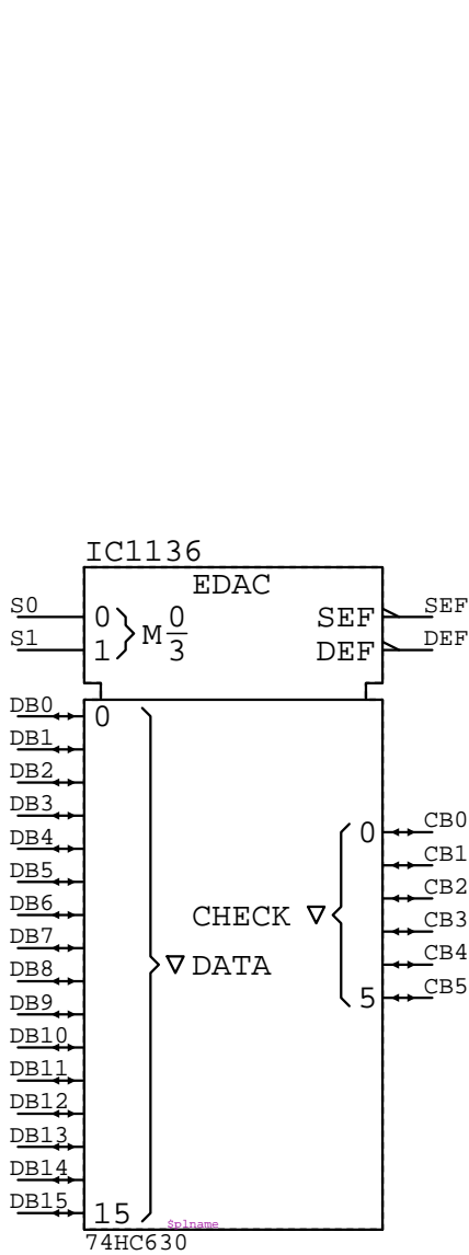
74HC630 IC????
