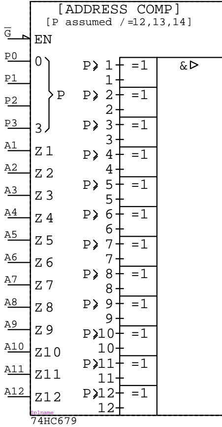
74HC679 IC?????
