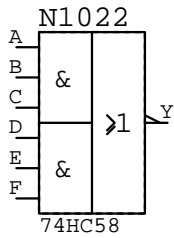
74HC58 N????
