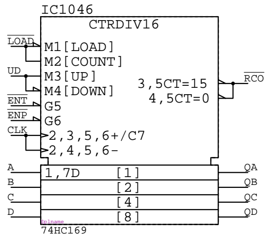
74HC169 IC????
