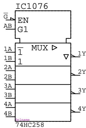
74HC258 IC????
