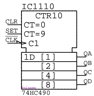
74HC490 IC????
