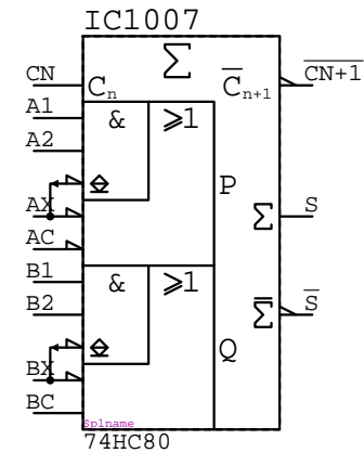
74HC80 IC????
