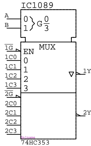
74HC353 IC????
