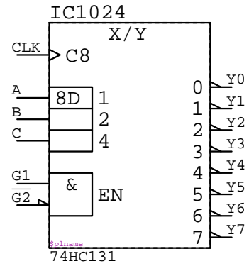
74HC131 IC????
