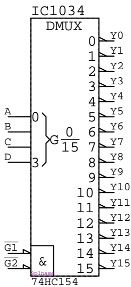
74HC154
