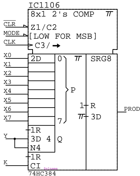
74HC384 IC????
