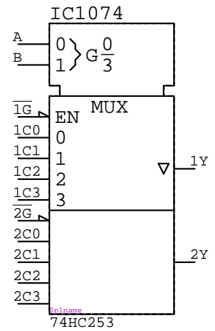
74HC253 IC????
