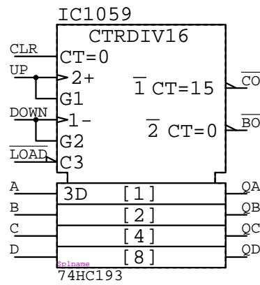
74HC193 IC?????
