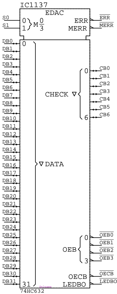
74HC632 IC????
