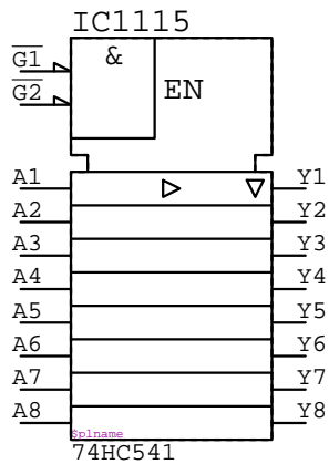
74HC541 IC?????
