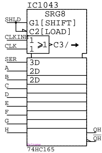
74HC165 IC????
