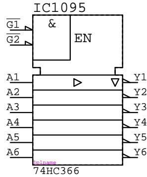
74HC366 IC?????
