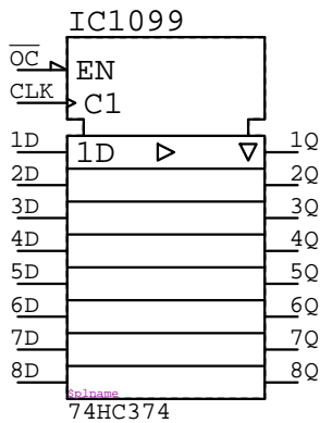
74HC374 IC?????
