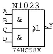
74HC58X N????
