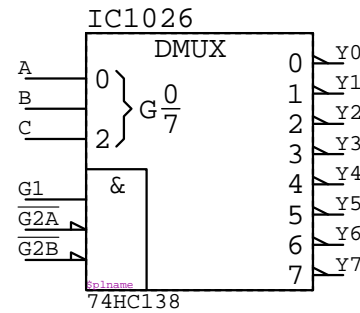
74HC138 IC????
