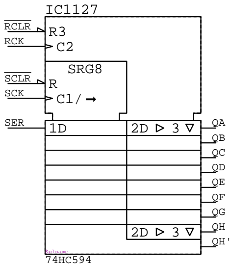
74HC594 IC????
