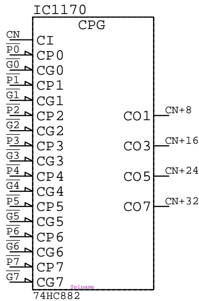
74HC882 IC????
