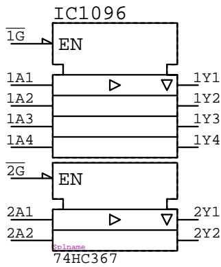
74HC367 IC?????
