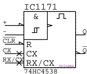
74HC4538 IC????
