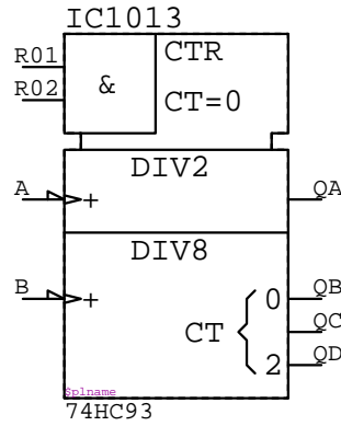
74HC93 IC????
