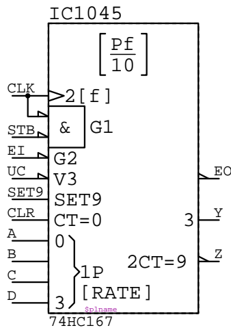
74HC167 IC????
