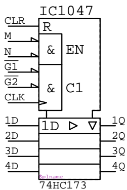
74HC173 IC????
