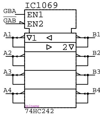
74HC242 IC????
