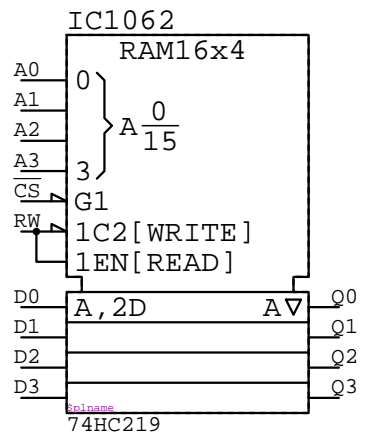
74HC219 IC?????
