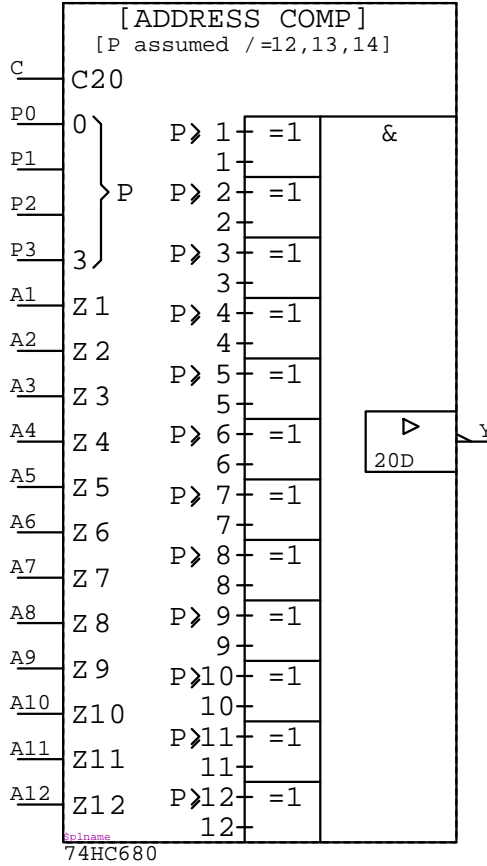
74HC680 IC?????
