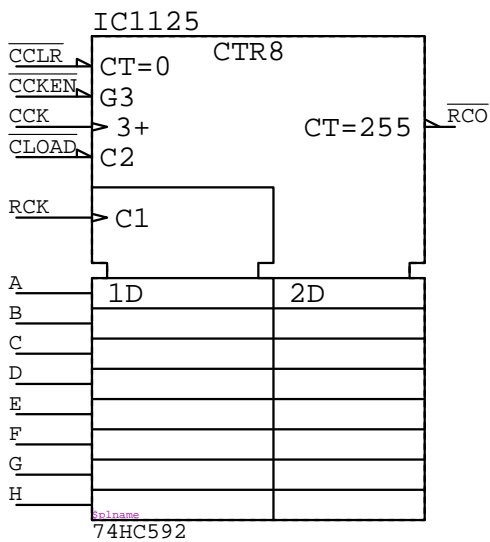
74HC592 IC????
