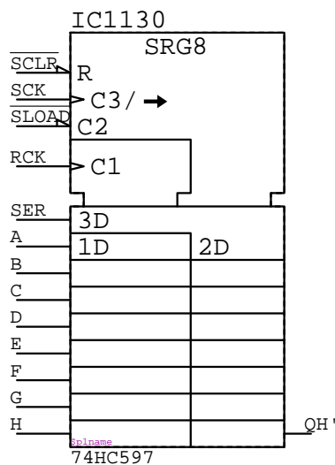
74HC597 IC????
