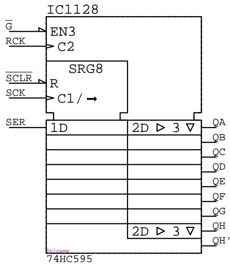
74HC595 IC????
