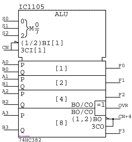
74HC382 IC????
