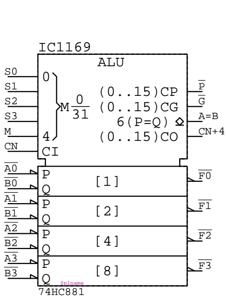
74HC881 IC????
