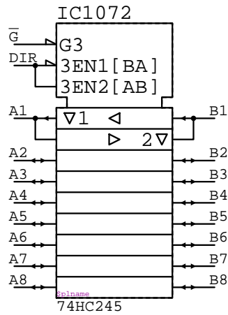
74HC245 IC????
