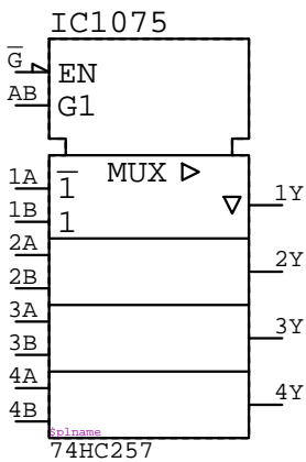
74HC257 IC????
