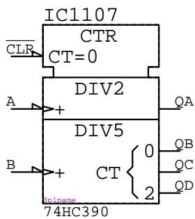
74HC390 IC????
