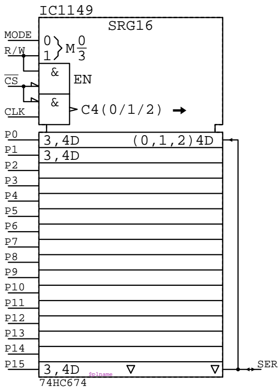
74HC674 IC????
