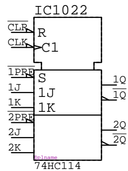
74HC114 IC????
