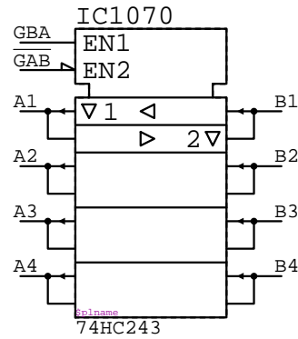
74HC243 IC????
