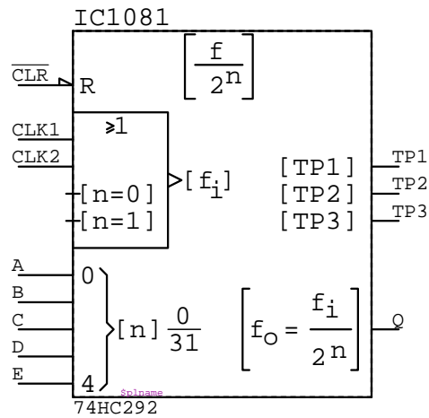
74HC292 IC?????
