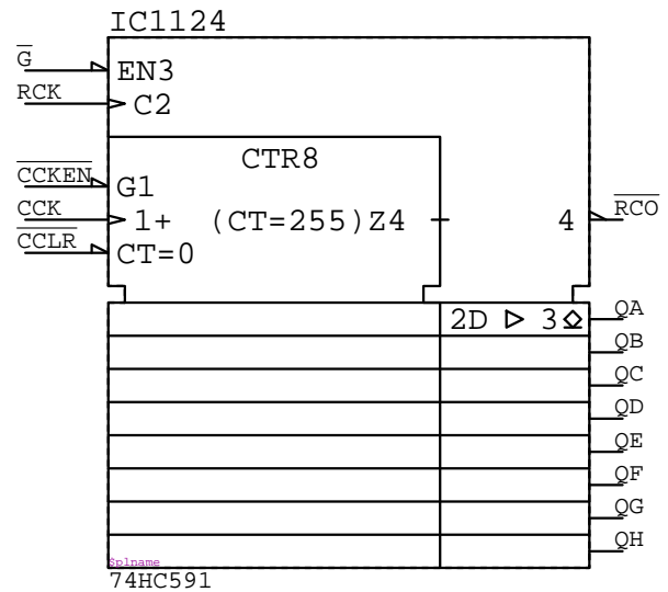
74HC591 IC????
