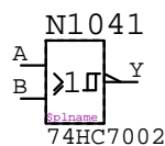
74HC7002 N????
