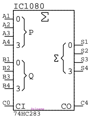
74HC283 IC?????
