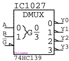
74HC139 IC????
