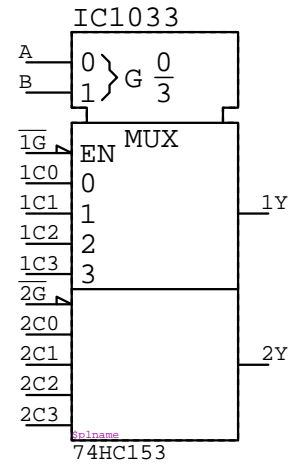
74HC153
