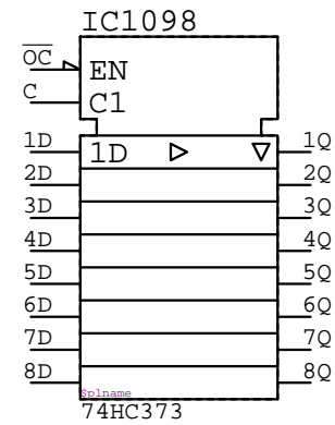
74HC373 IC?????
