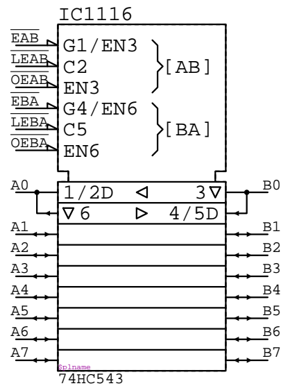
74HC543 IC?????
