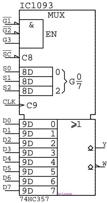
74HC357 IC?????
