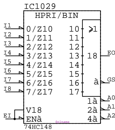
74HC148 IC????
