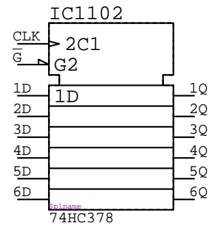
74HC378 IC?????
