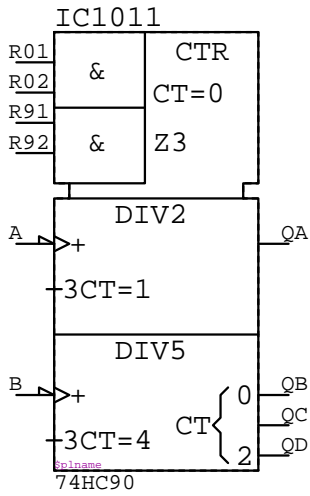
74HC90 IC????
