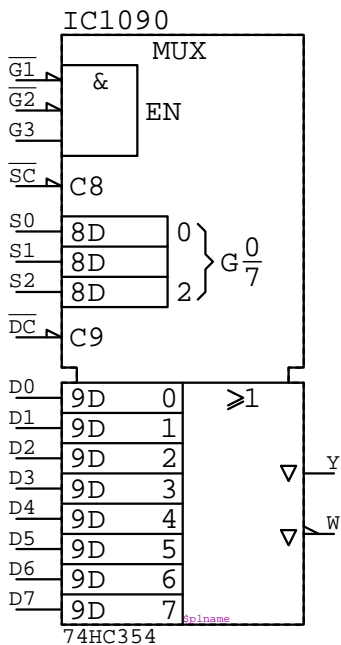
74HC354 IC????
