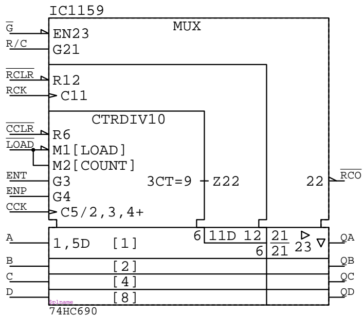
74HC690 IC????
