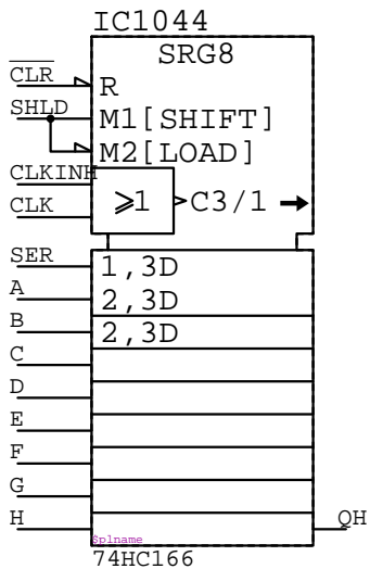
74HC166 IC????
