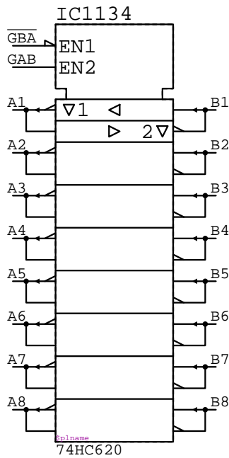
74HC620 IC?????
