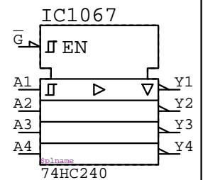
74HC240 IC?????
