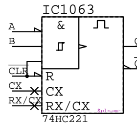
74HC221 IC?????
