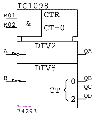
74293 IC????
