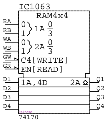
74170 IC????
