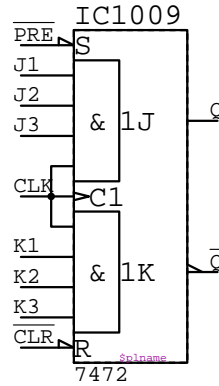
7472 IC????
