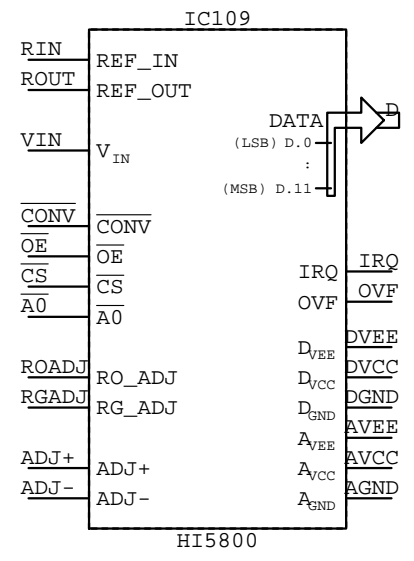
HI5800 IC???
