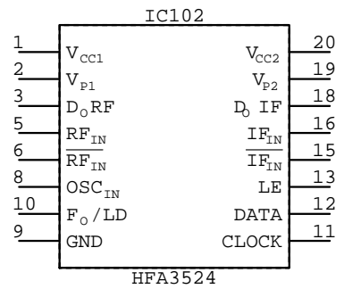
HFA3524 IC???
