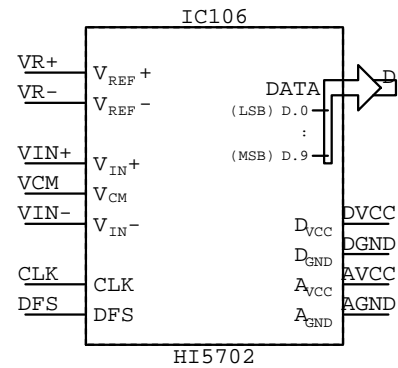
HI5702 IC???
