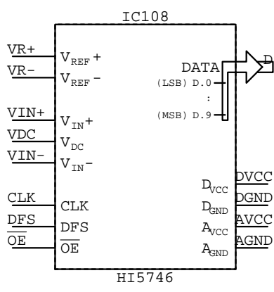
HI5746 IC???
