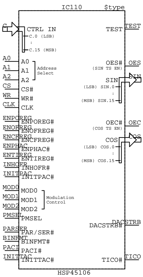
HSP45106 IC???
