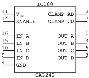
CA3242 IC???
