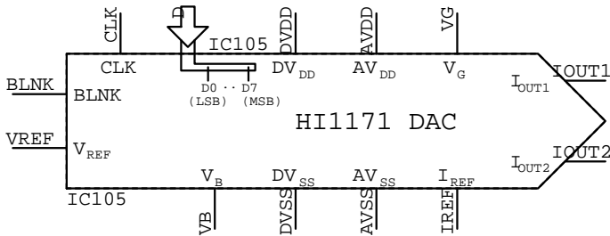
HI1171 IC???
