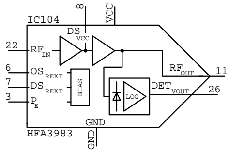
HFA3983 IC???
