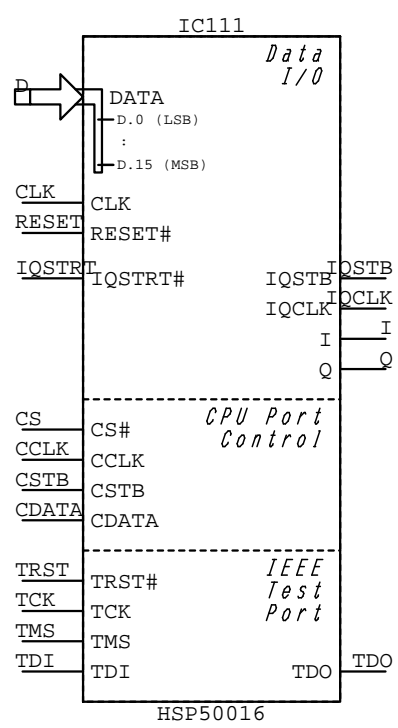
HSP50016 IC???
