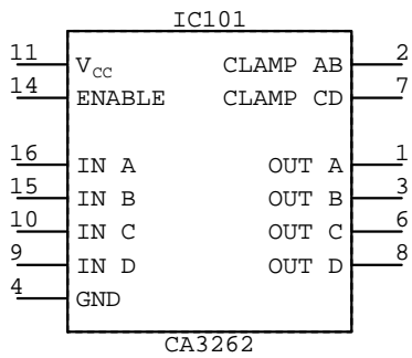
CA3262 IC???
