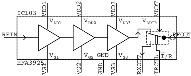
HFA3925 IC???
