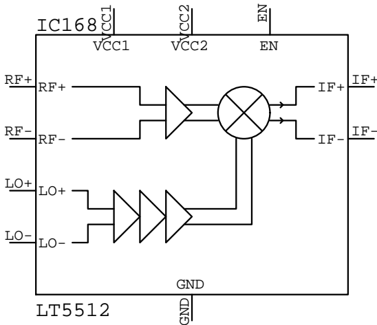
LT5512 IC???
