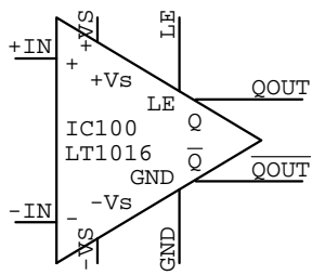
LT1016 IC???
