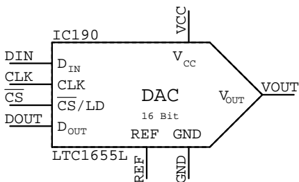
LTC1655L IC???
