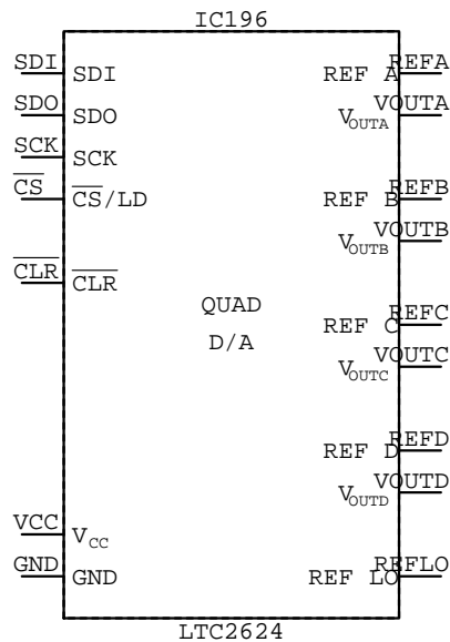
LTC2624 IC???
