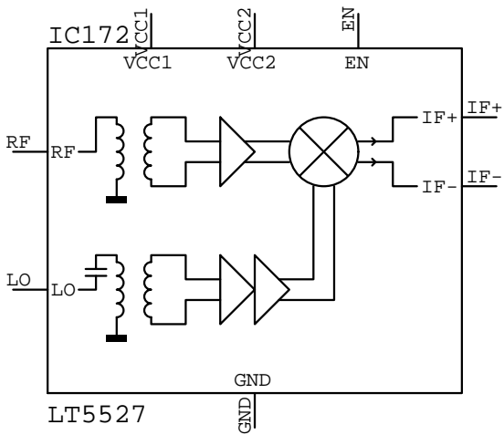
LT5527 IC???
