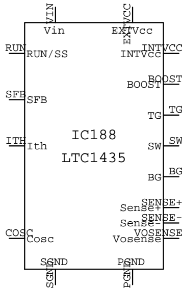
LTC1435 IC???
