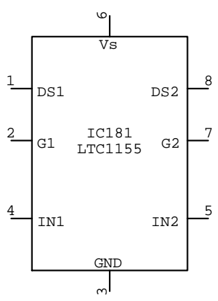
LTC1155 IC???
