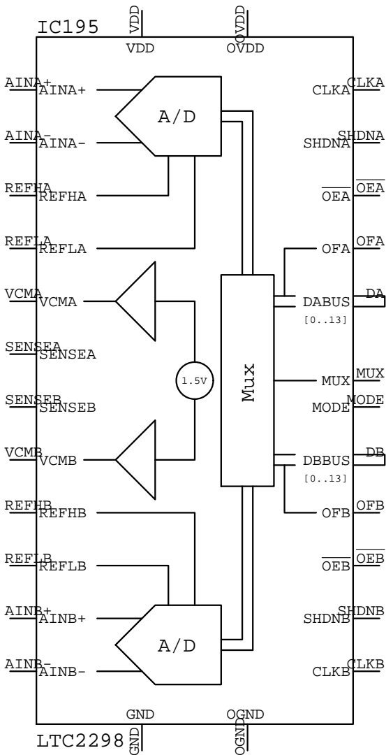
LTC2298 IC???
