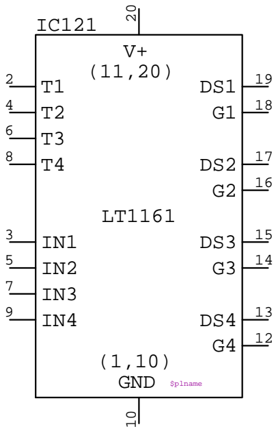
LT1161 IC???
