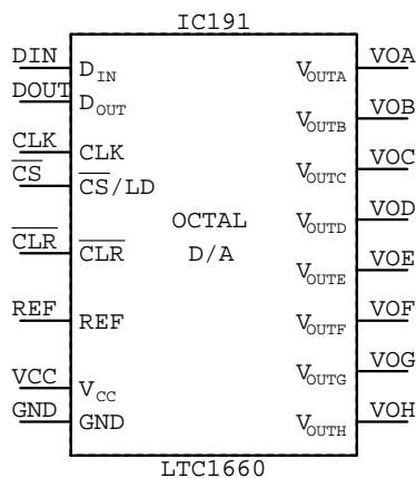
LTC1660 IC???
