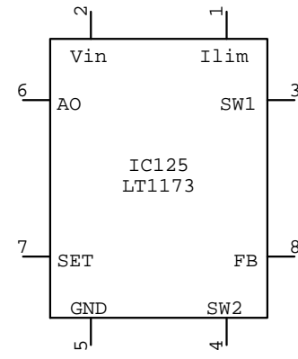
LT1173 IC???
