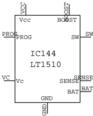
LT1510_CS8 IC???
