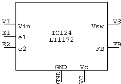
LT1172 IC???
