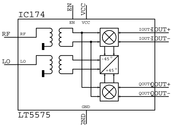
LT5575 IC???
