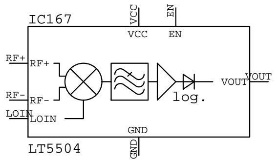
LT5504 IC???
