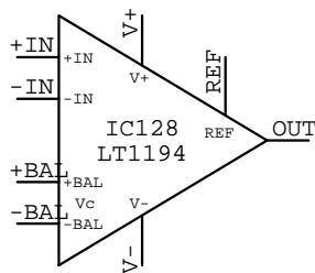
LT1194 IC???
