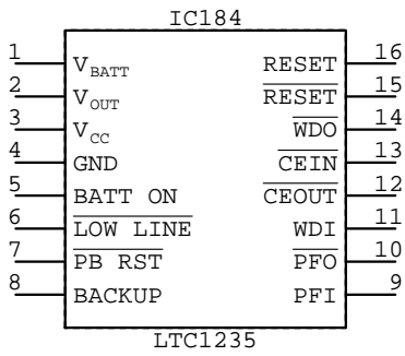
LTC1235 IC???
