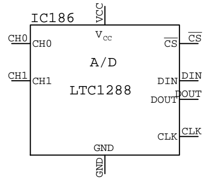
LTC1288 IC???
