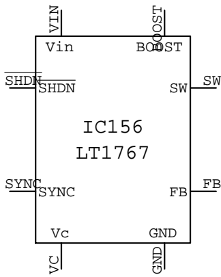
LT1767 IC???
