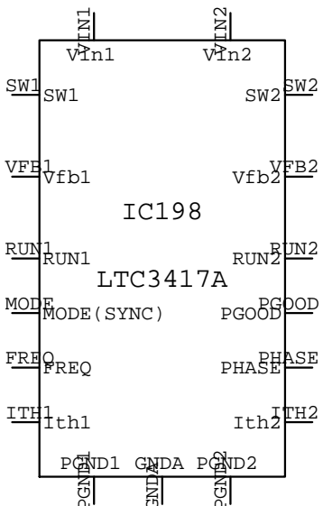
LTC3417_FE IC???
