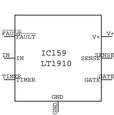
LT1910 IC???
