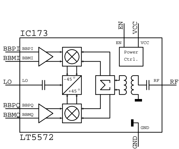
LT5572 IC???
