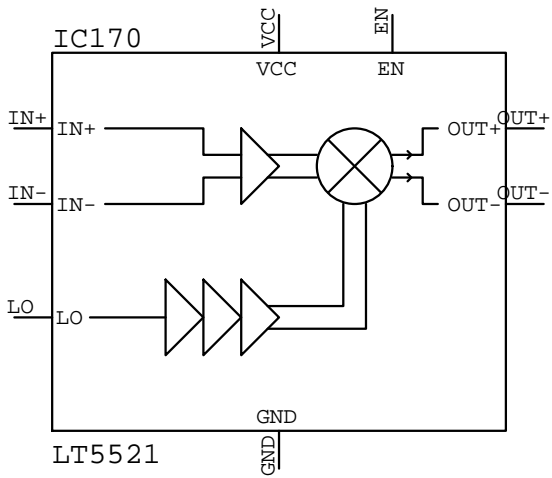
LT5521 IC???
