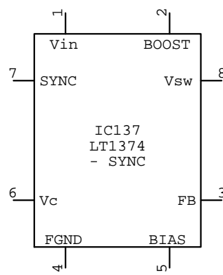
LT1374_S_SO IC???
