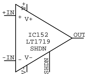
LT1719S6 IC???
