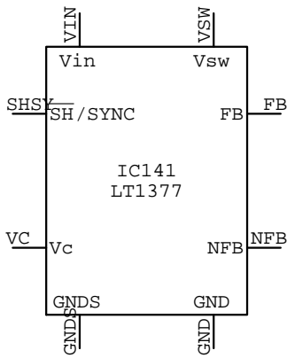
LT1377 IC???
