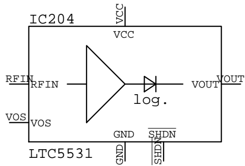
LTC5531 IC???
